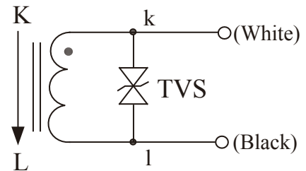
TVS: Transient voltage suppressor,Current output type
