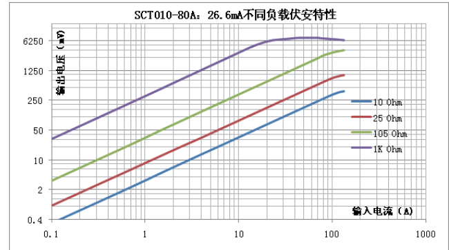
Characteristic curve in different load volt-ampere:
