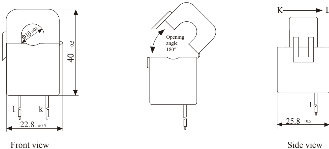
Outline size diagram(in mm):
